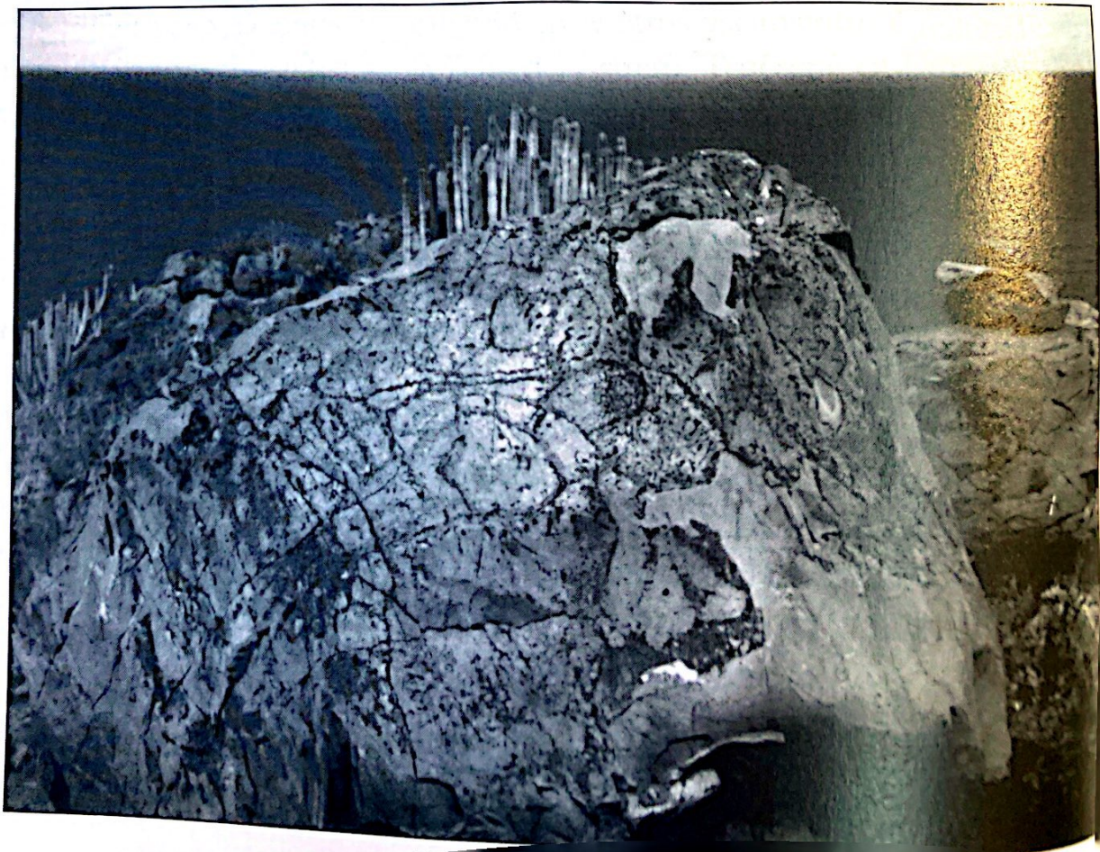
Tamadite, Tenerife
